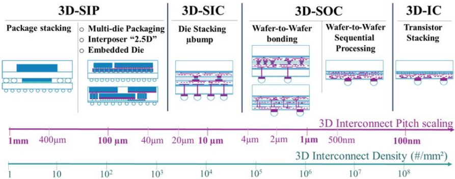
Figure 1.3.4 3D landscape, ordering of 3D technologies according to the system-level wiring hierarchy [11] [12].
